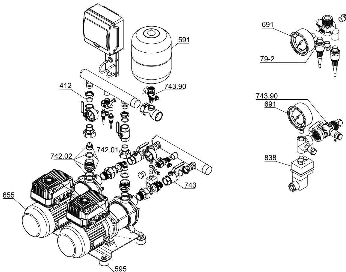
Fig. 14: DeltaBasic Compact MVP
