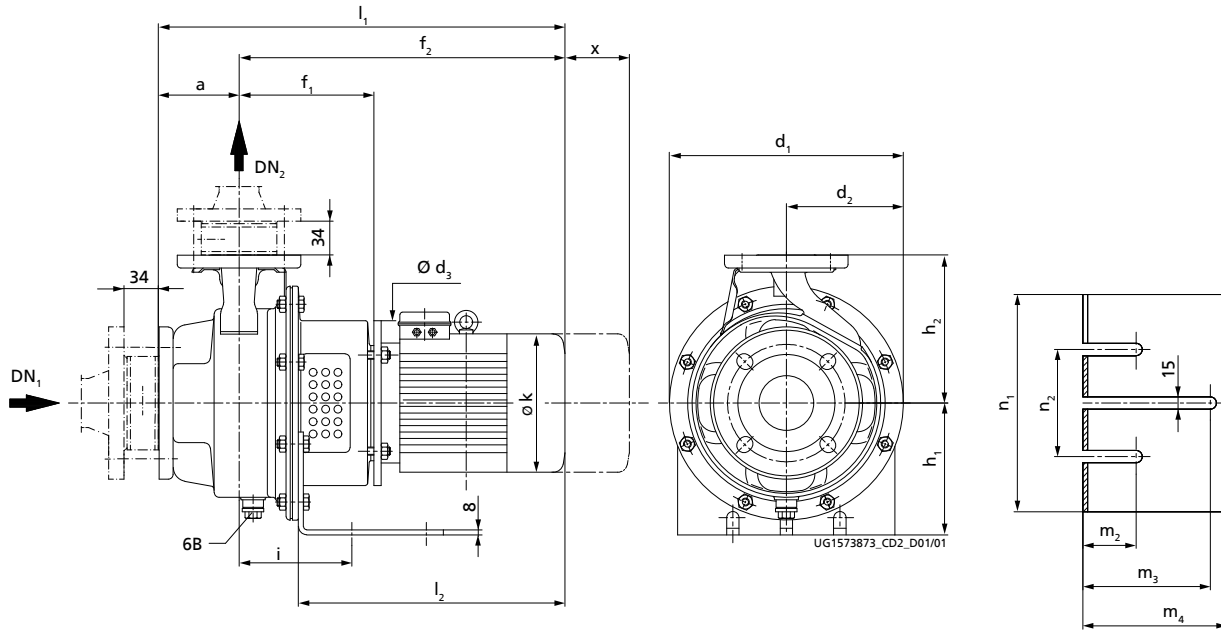
Fig. 5: Etachrom B with pump foot, dimensions [mm]
